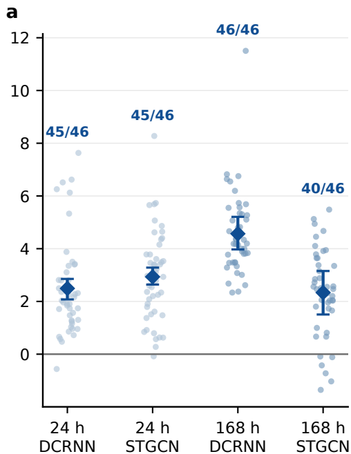
Publisher-compatible MAE improvement (baseline – STaR-GNN; \text{L s}^{-1} )
