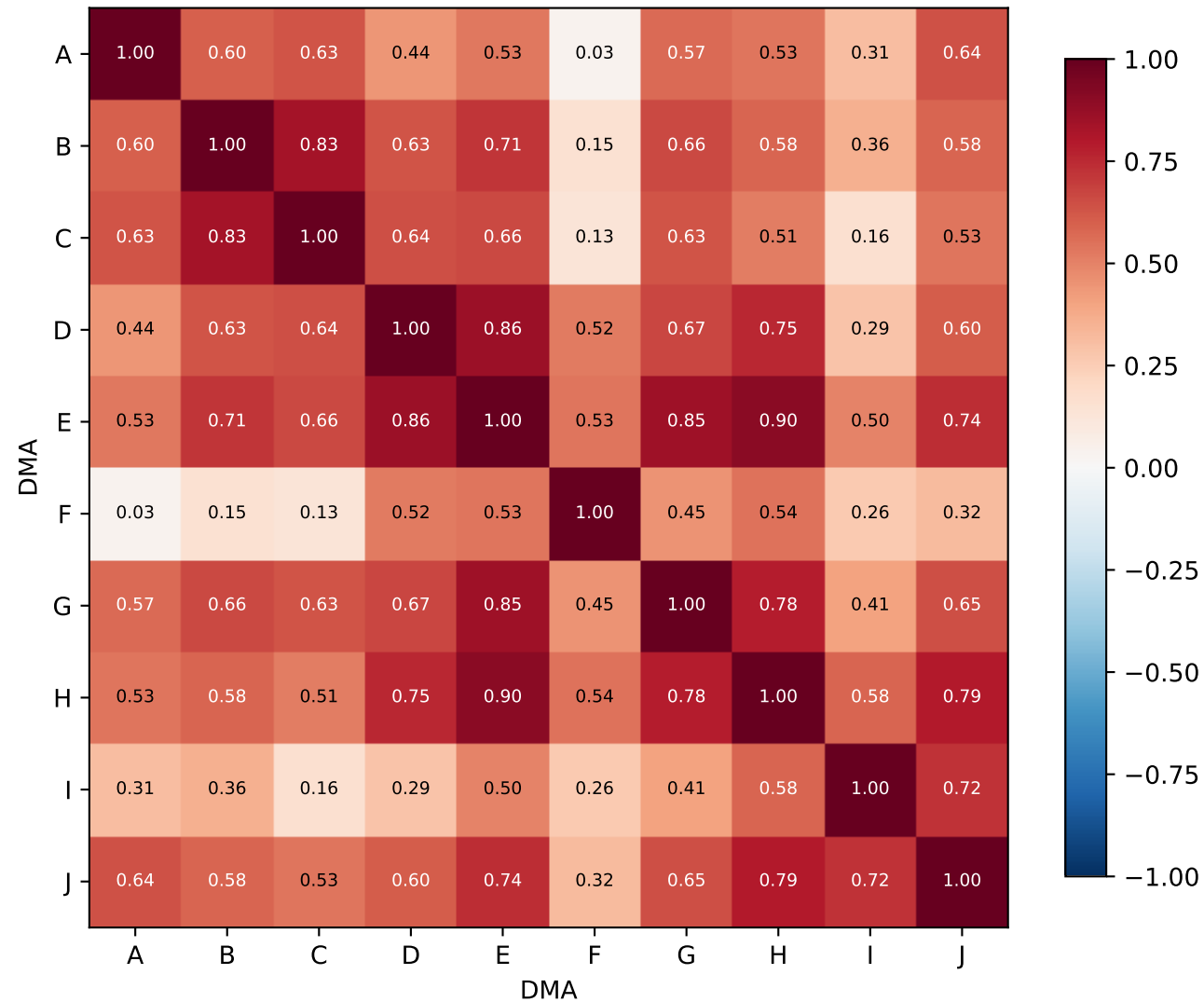
Training-period Pearson functional graph
