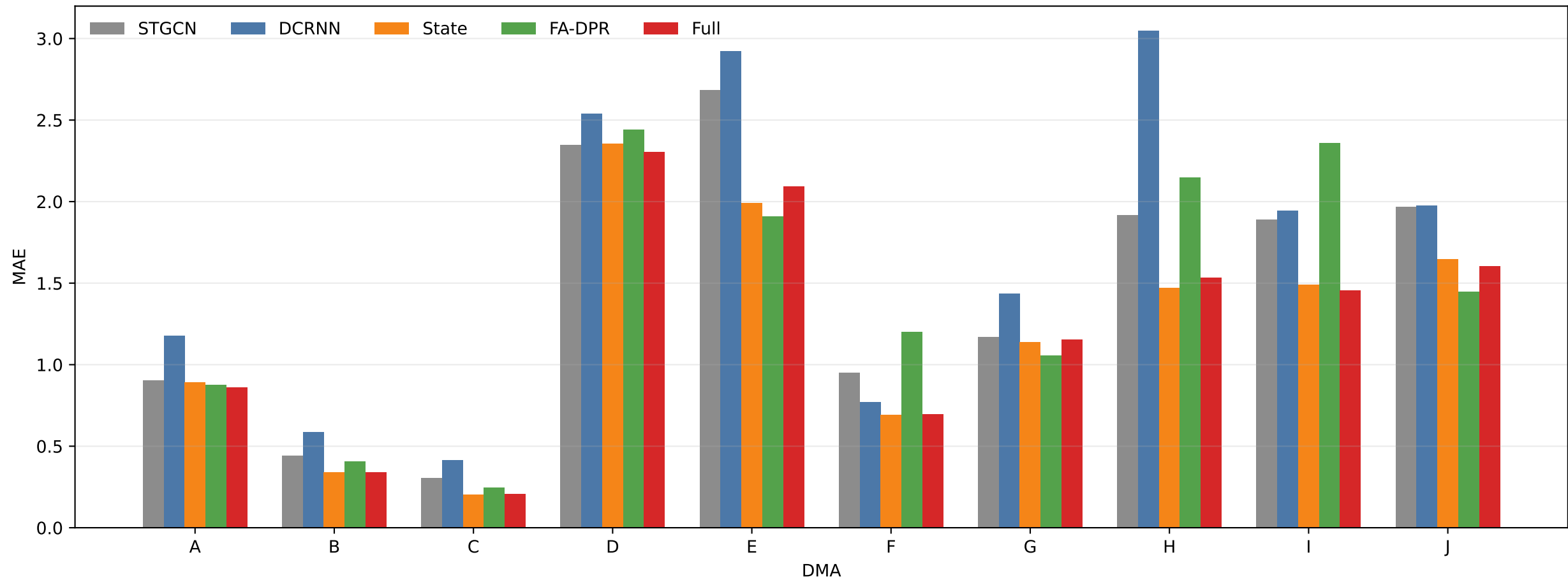
DMA-level common-46 Test MAE (168h)
