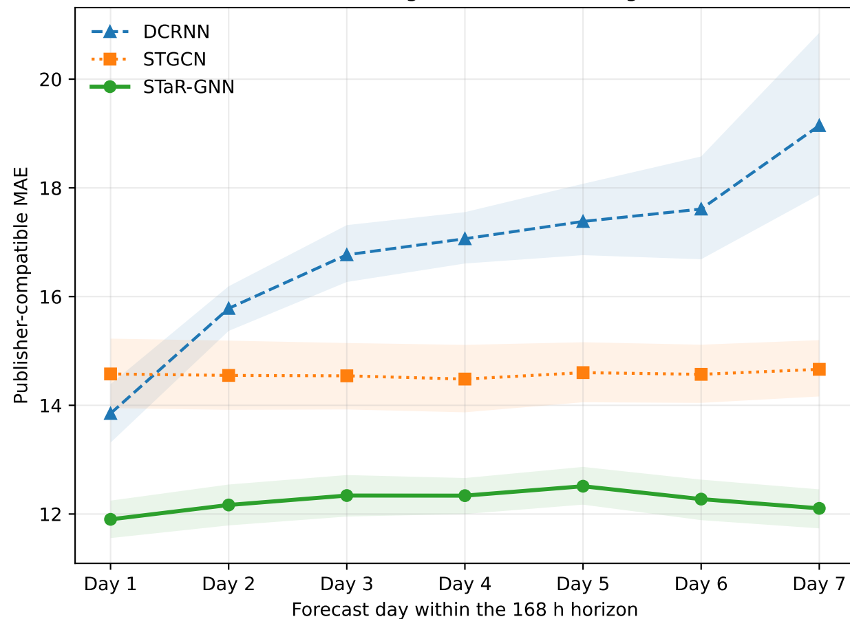
(a) Absolute long-horizon forecasting error
