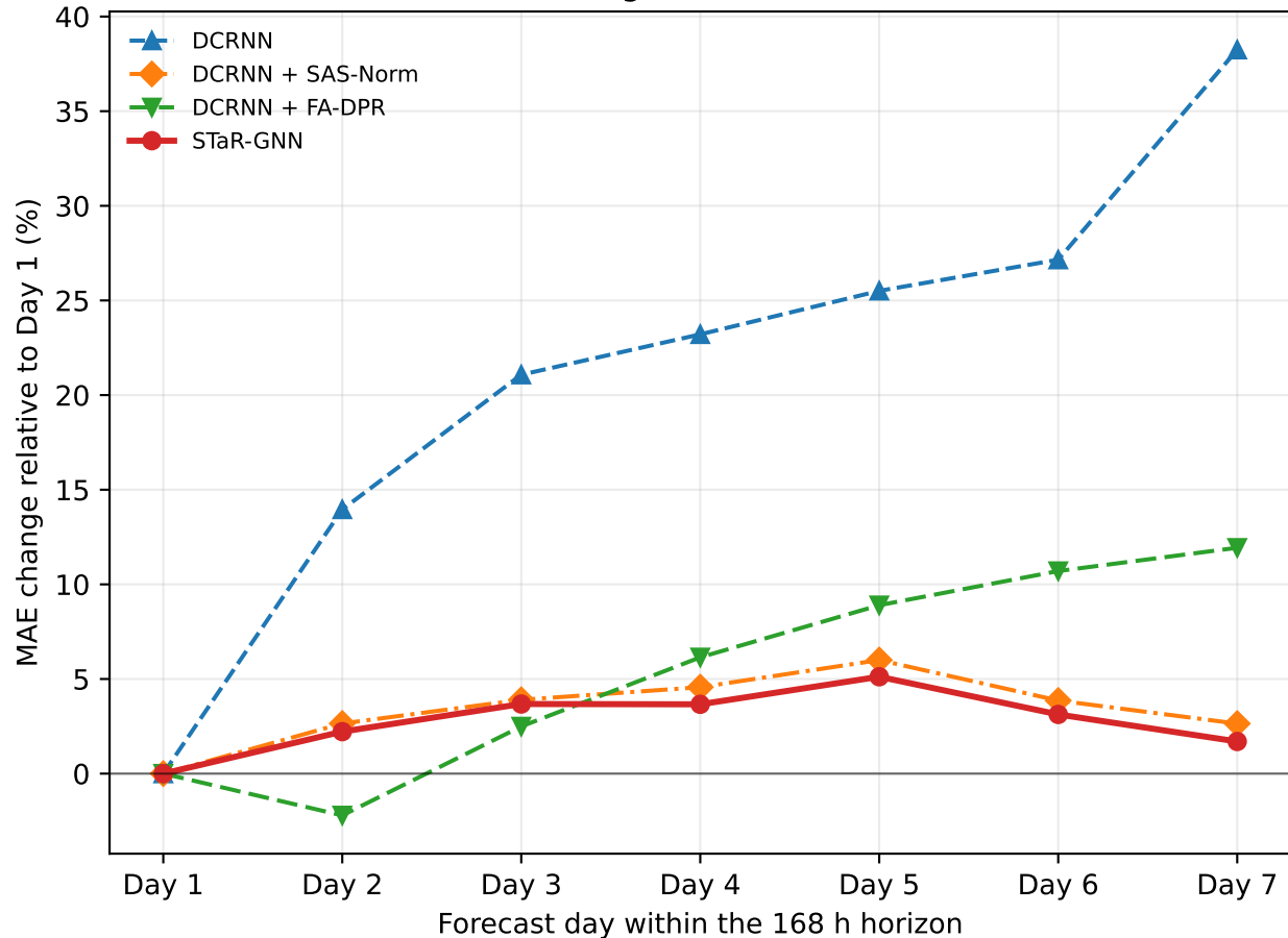
(b) Relative error degradation of ablation variants
