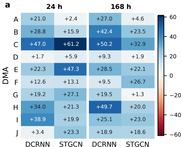
RMSE reduction (%)
