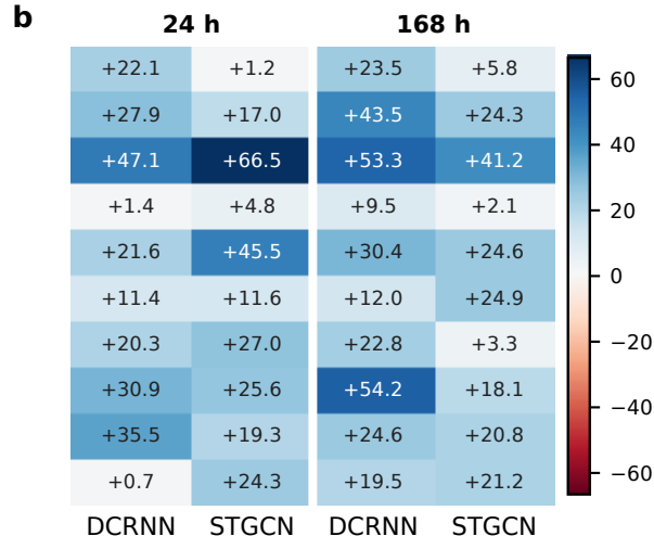
NSE gain
