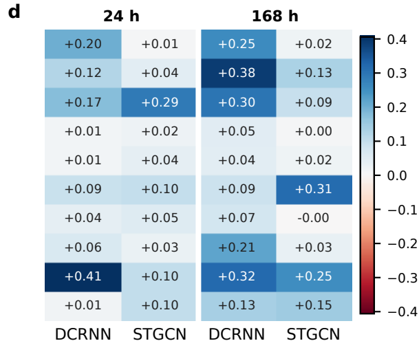
NSE gain
