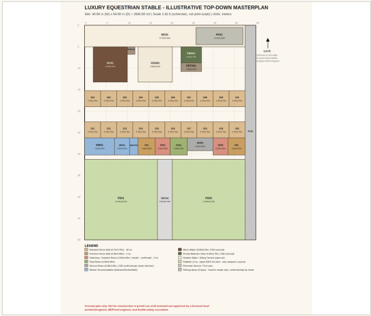
5. Styled Masterplan (SVG render)
