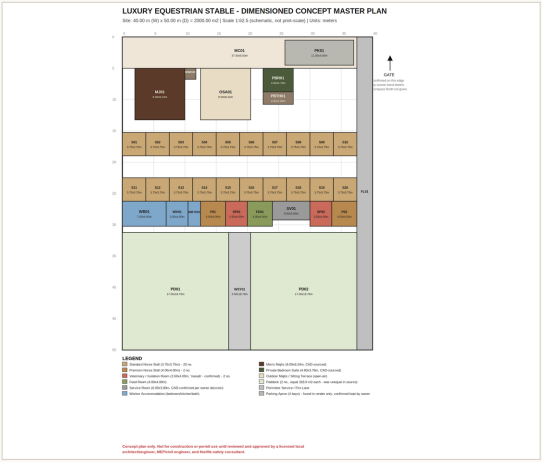
4. Dimensioned Technical Plan
