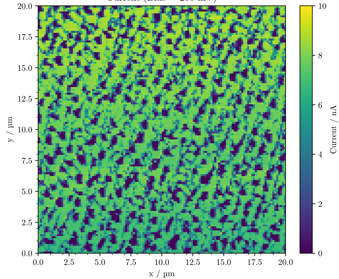
Current (Bias = 200 mV)
