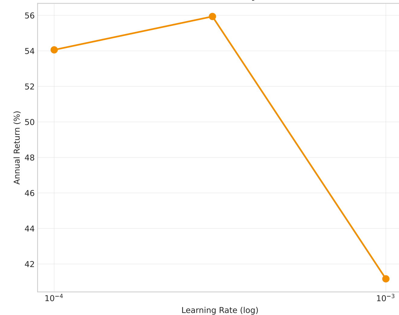
LR Sensitivity
