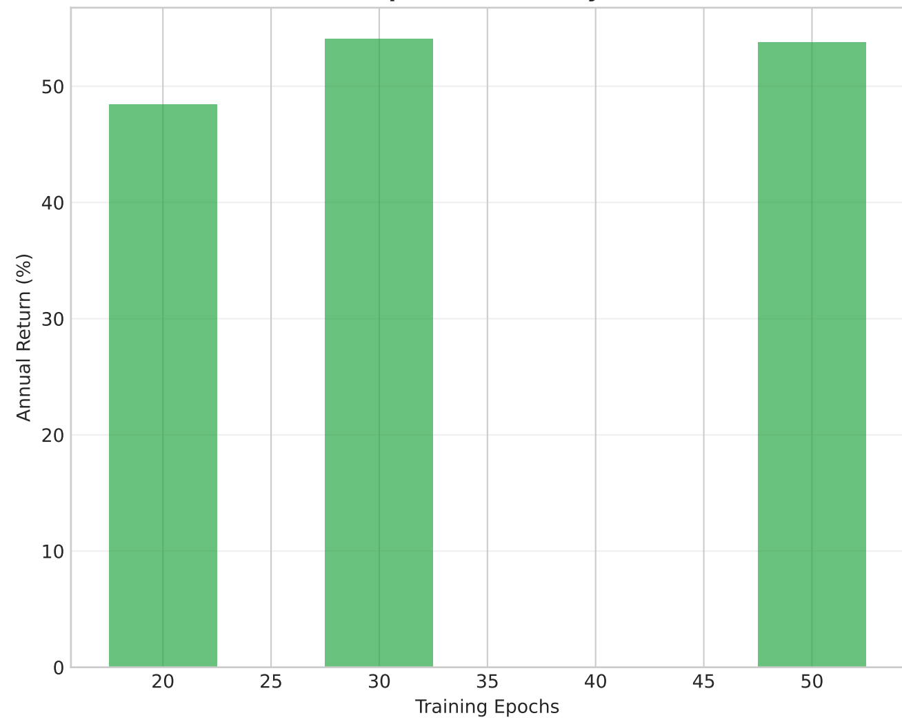
Epochs Sensitivity
