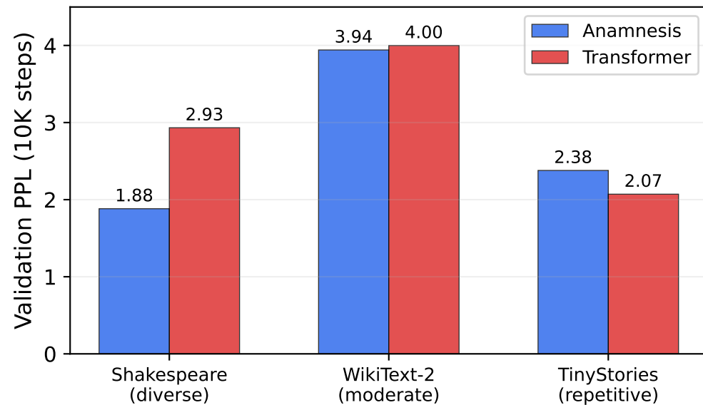
(a) Cross-Dataset PPL ( d = 128 )
