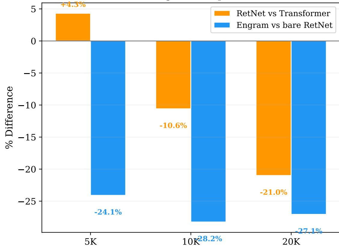
Advantage Decomposition
