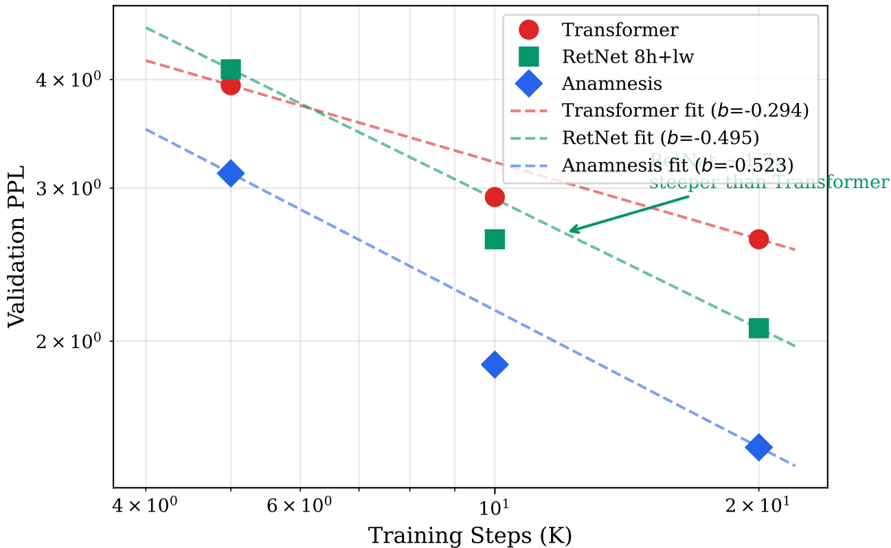
Scaling Law: \text{PPL} \propto \text{steps}^b (Shakespeare char-level, d=128 , \text{lr}=10^{-3} , seed=42)
