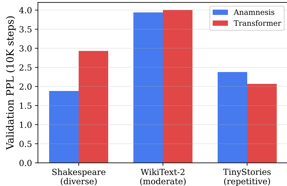
10K PPL by Dataset (d=128)
