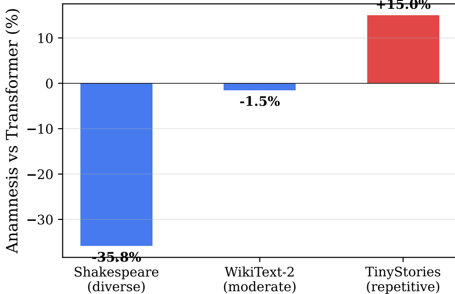
Advantage vs Data Diversity
