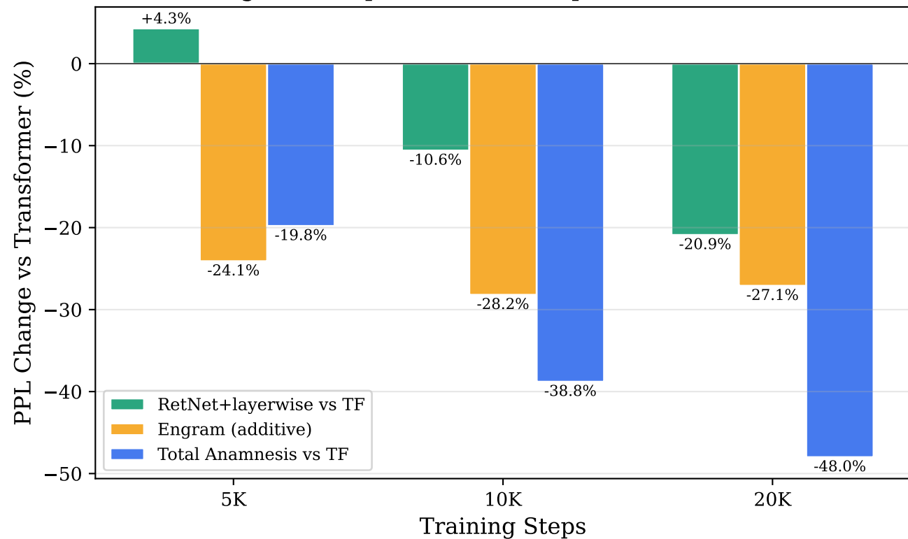
Advantage Decomposition (Shakespeare d=128, seed=42)
