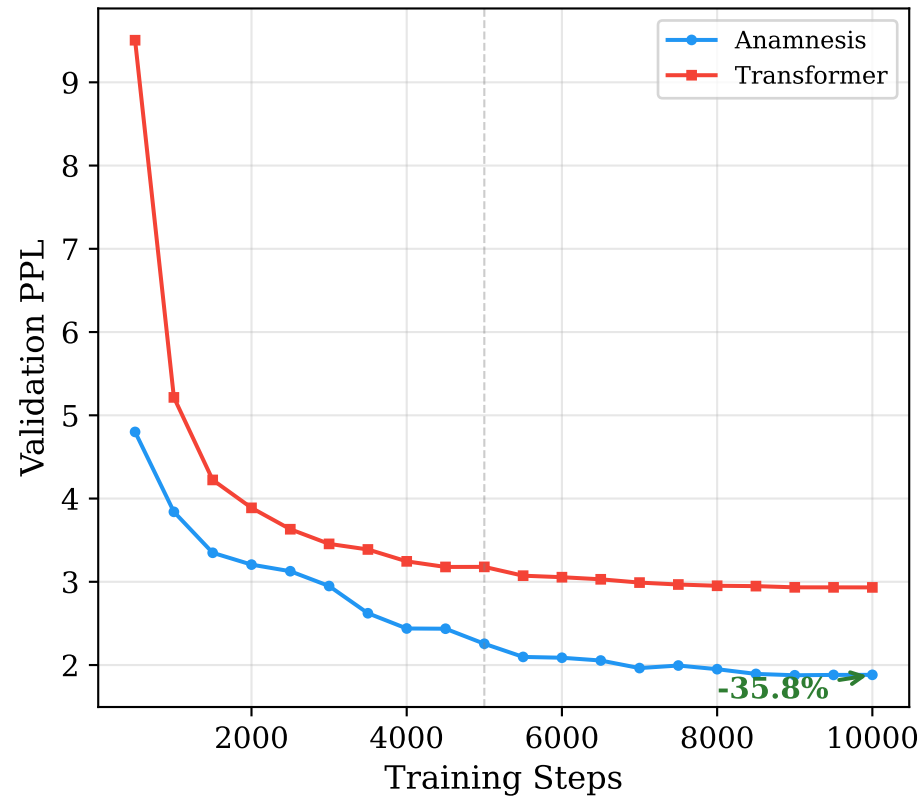
Shakespeare
