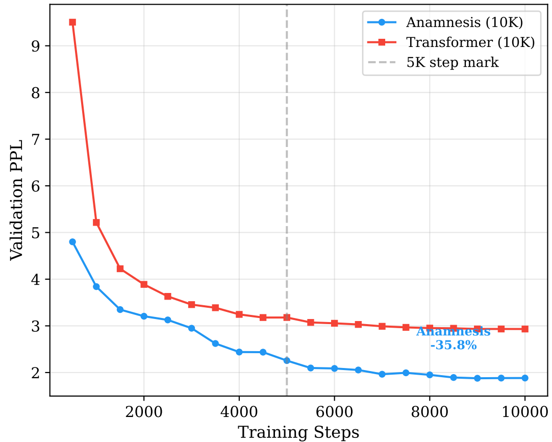
Validation PPL — Shakespeare char-level
