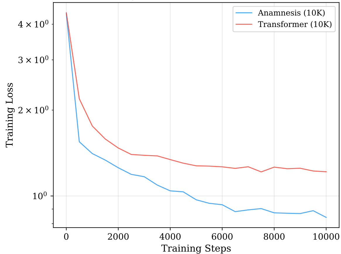
Training Loss — Shakespeare char-level
