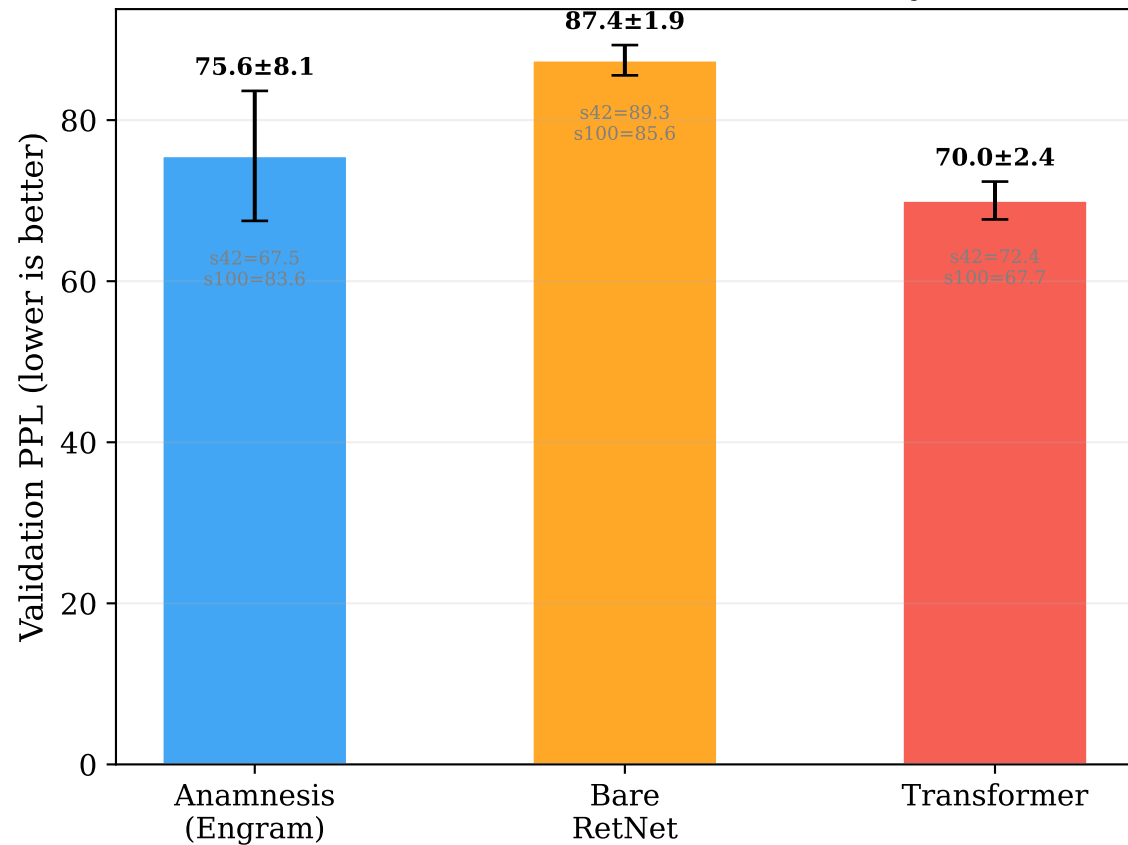
BPE WikiText-2: Seed Variance Analysis
