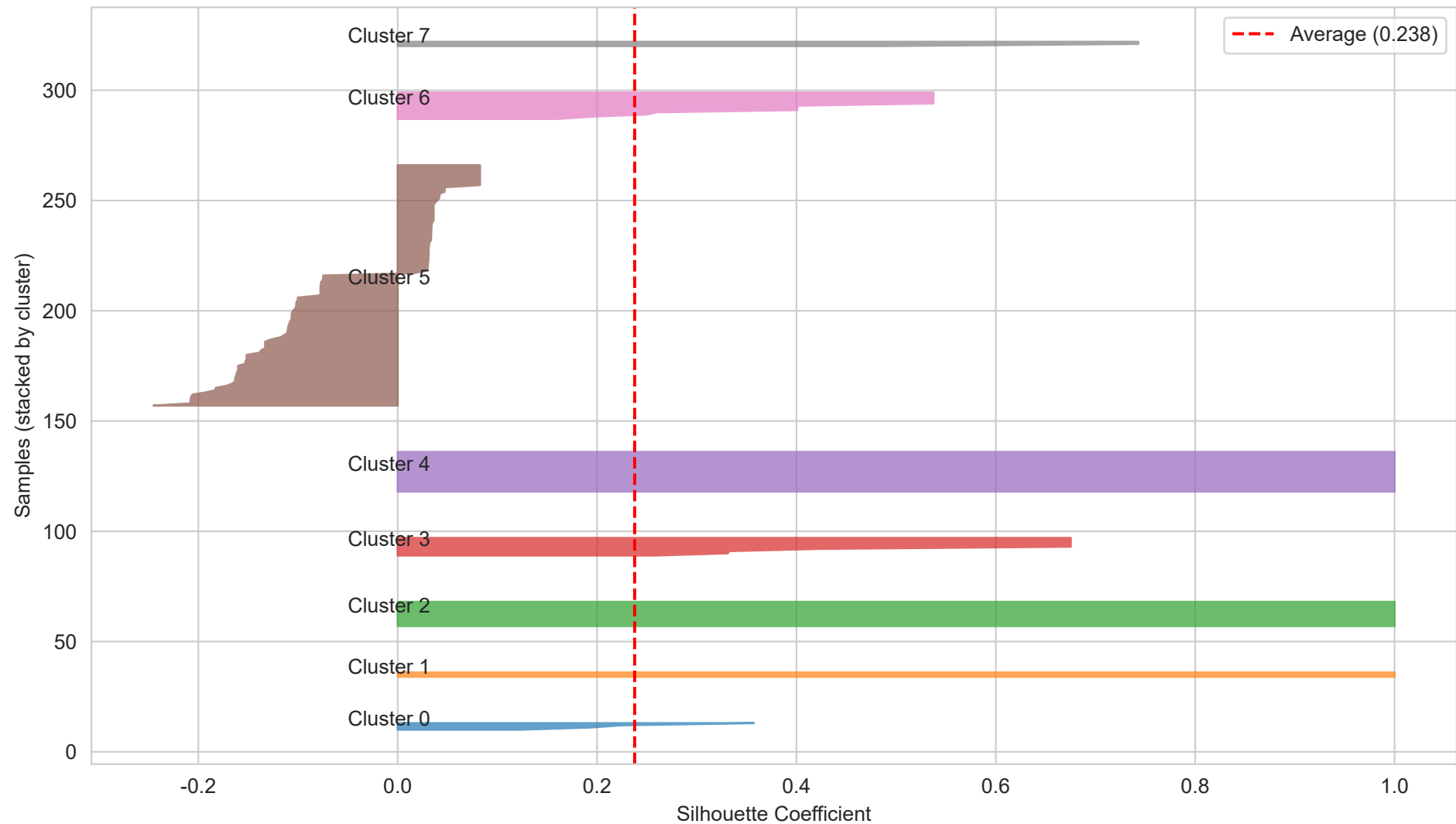
Silhouette Analysis for k=8
