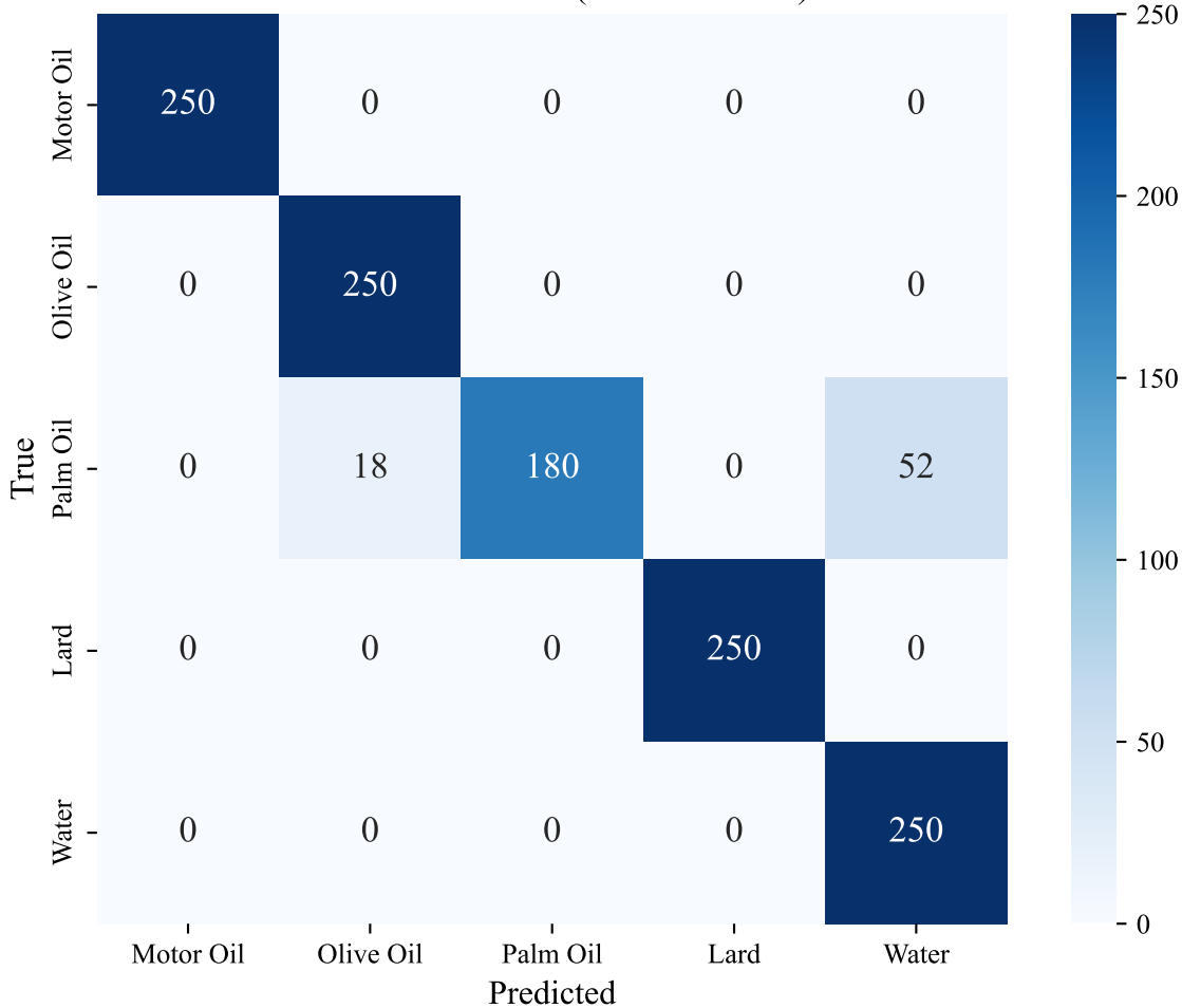
Confusion Matrix (Acc = 94.40%)
