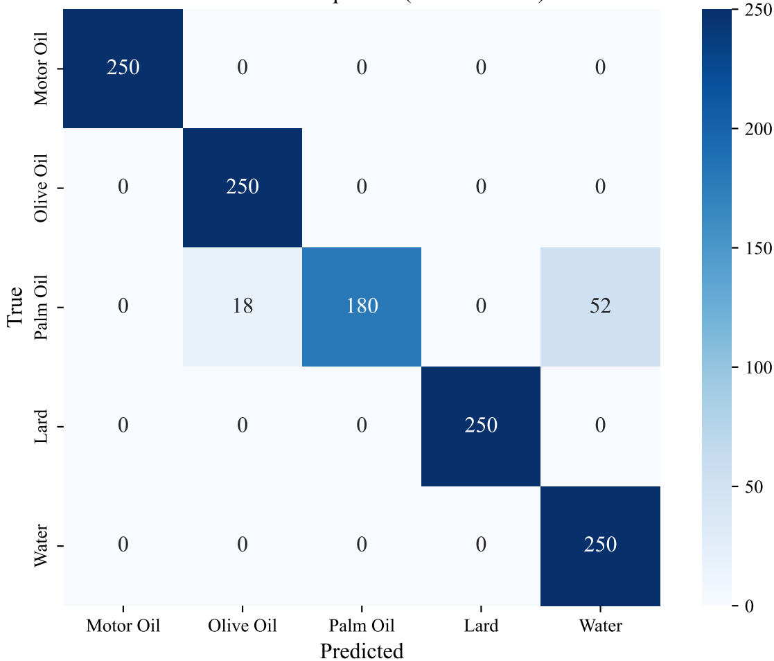
Held-out Real Spectra (Acc = 94.4%)
