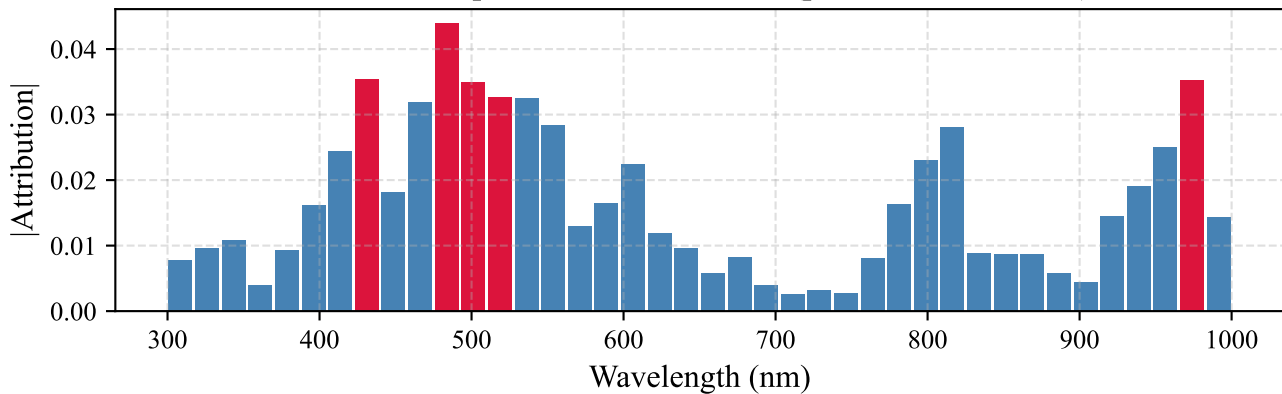
IG Band Importance — Olive Oil (predicted: Olive Oil)
