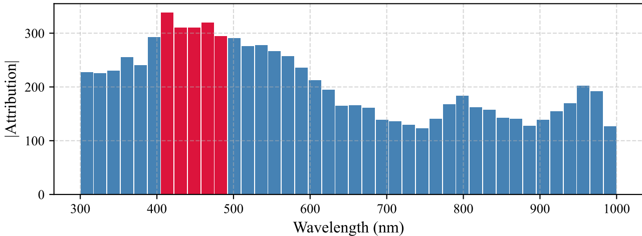
Integrated Gradients — Band Importance (Palm Oil)
