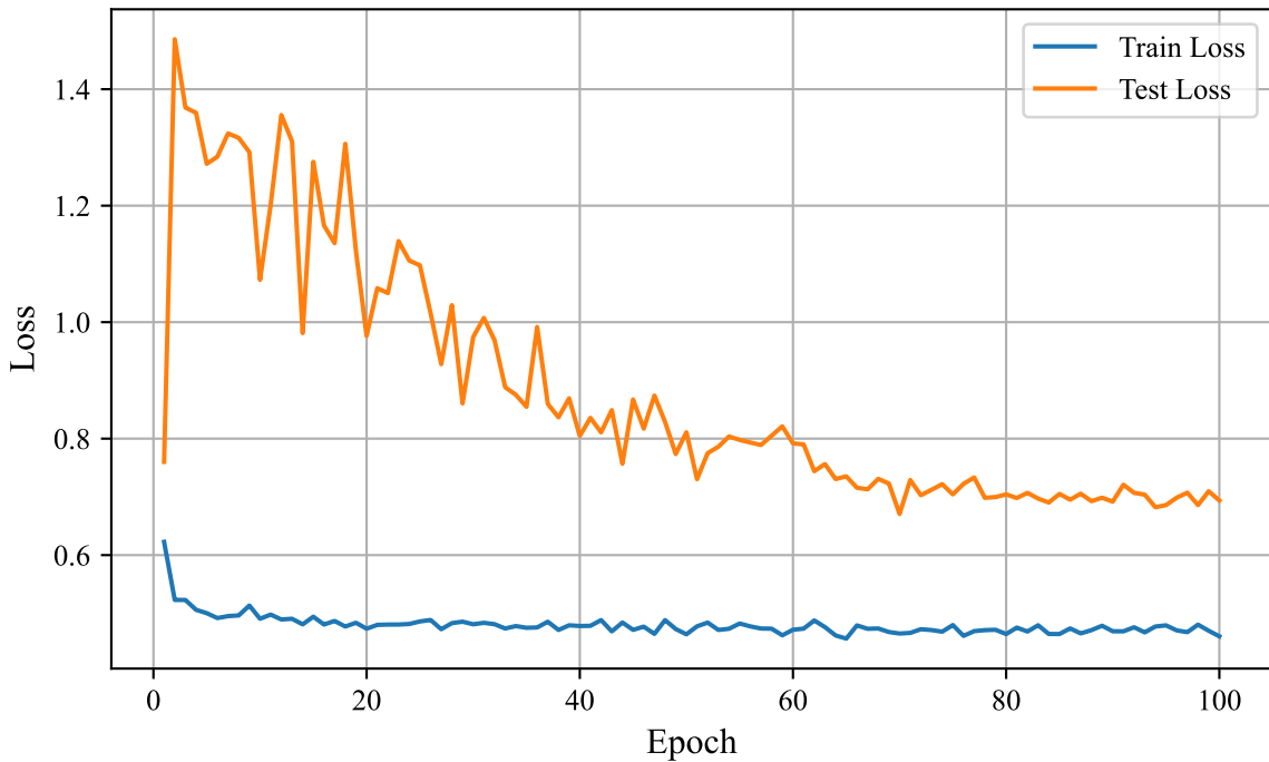
Train and Test Loss Curve
