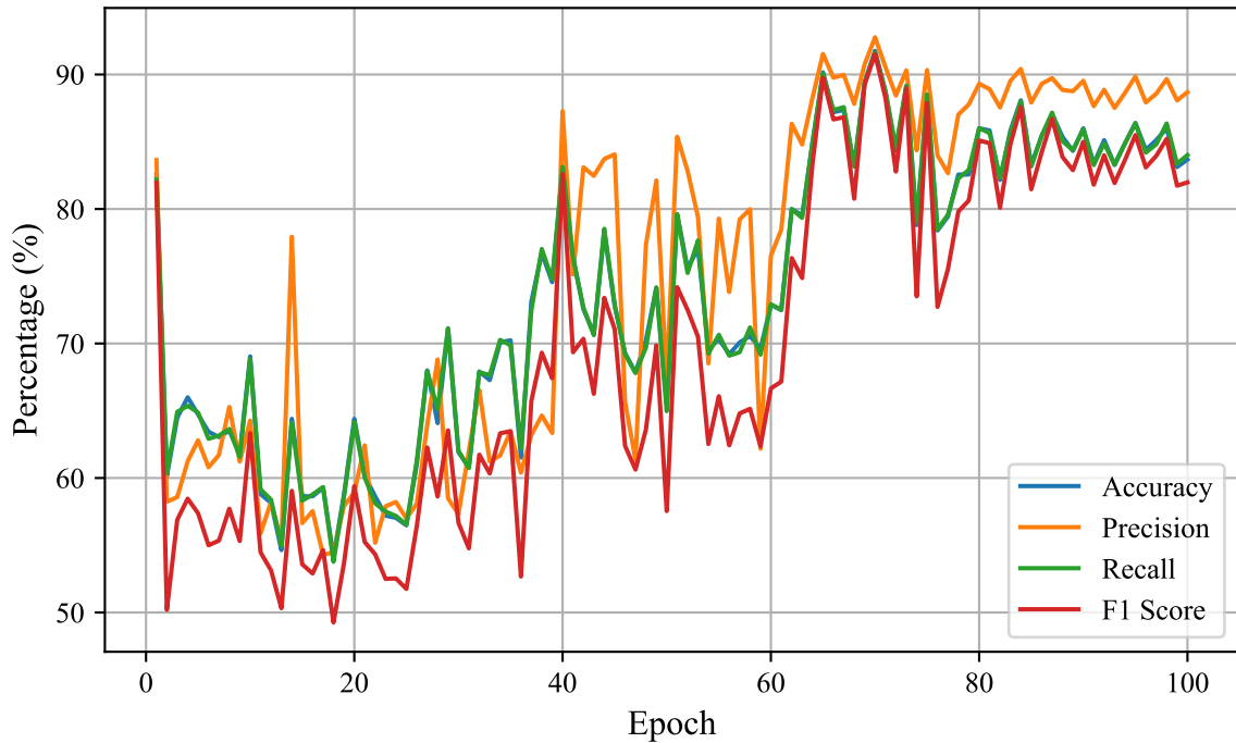
Overall Accuracy, Precision, Recall, and F1 Score
