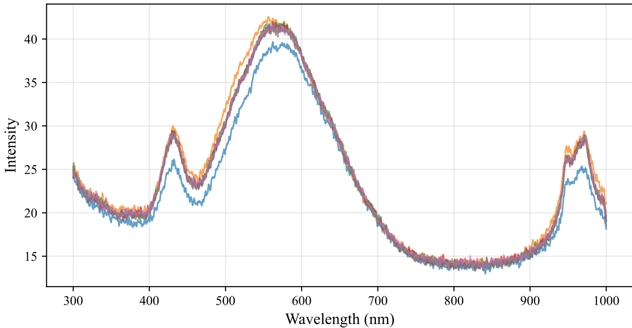
Motor Oil — Real Spectrum
