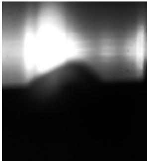
Olive Oil — Real
