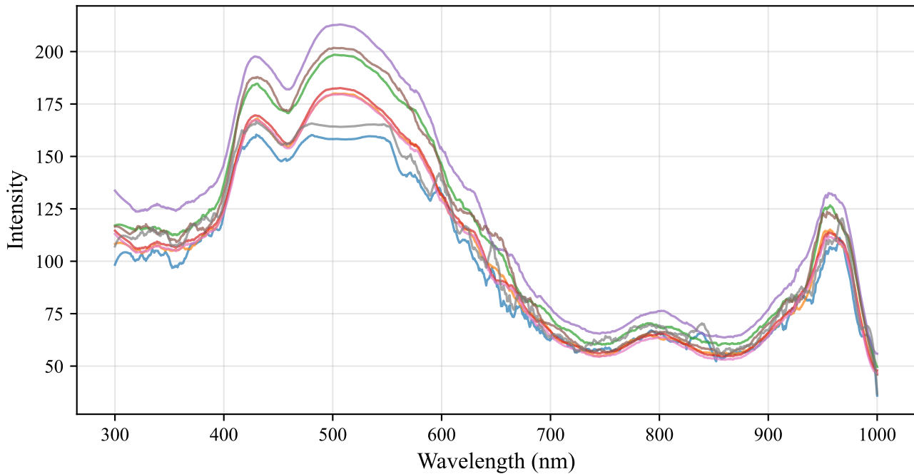
Olive Oil — CGAN Generated Spectrum
