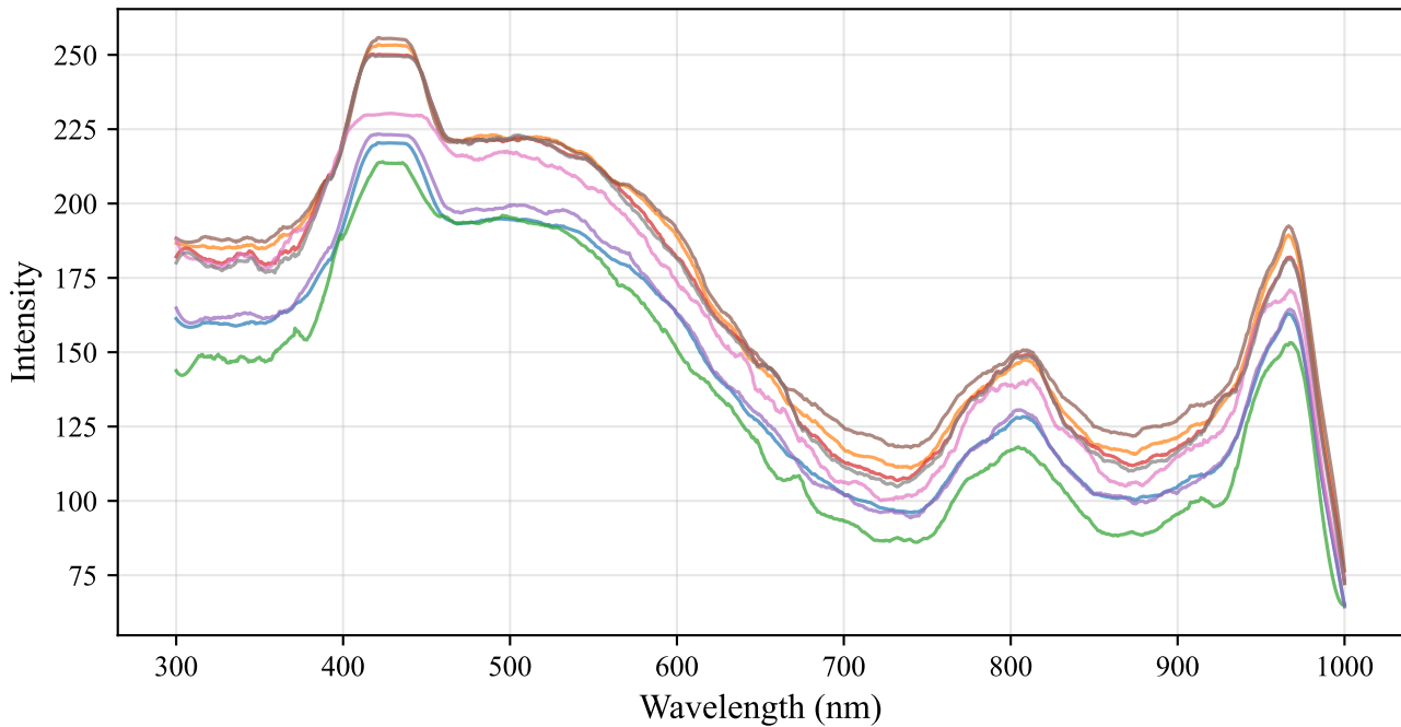
Water — CGAN Generated Spectrum
