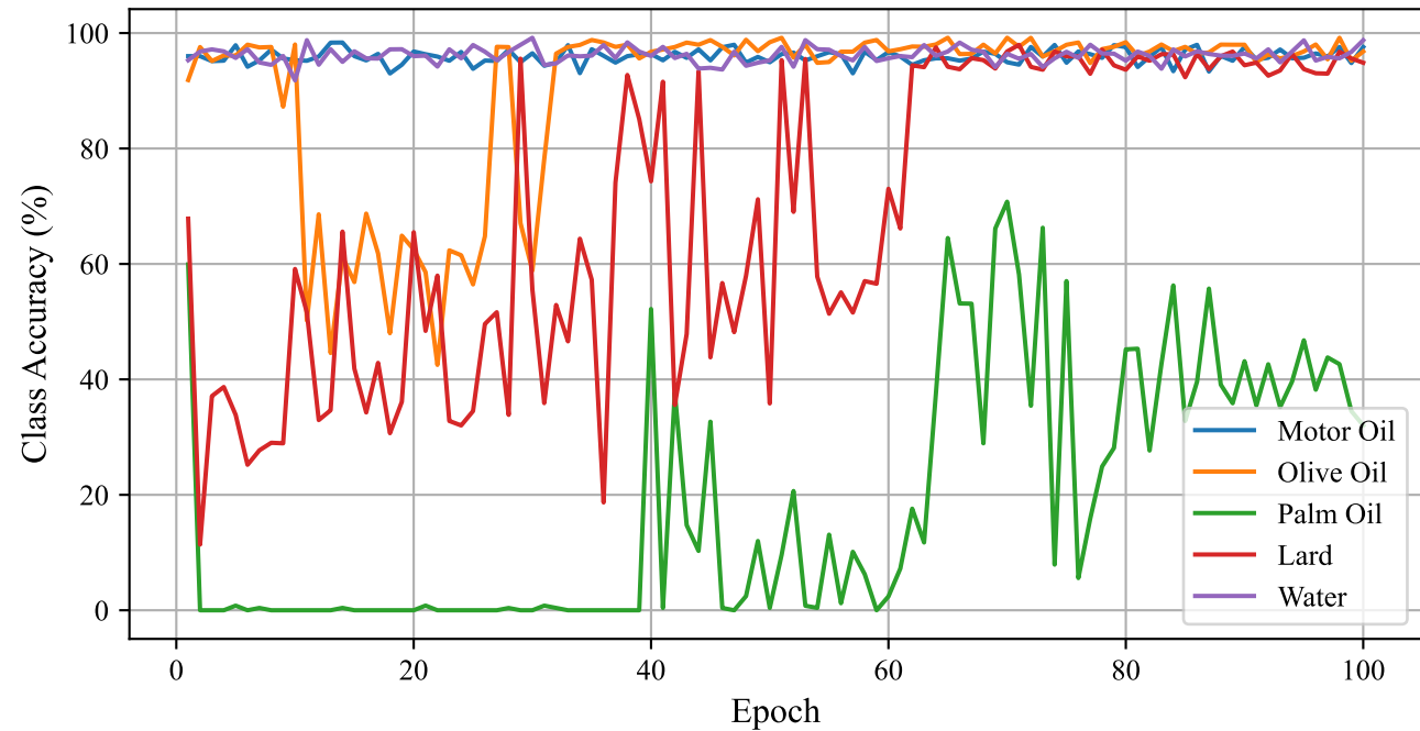
Class Accuracy
