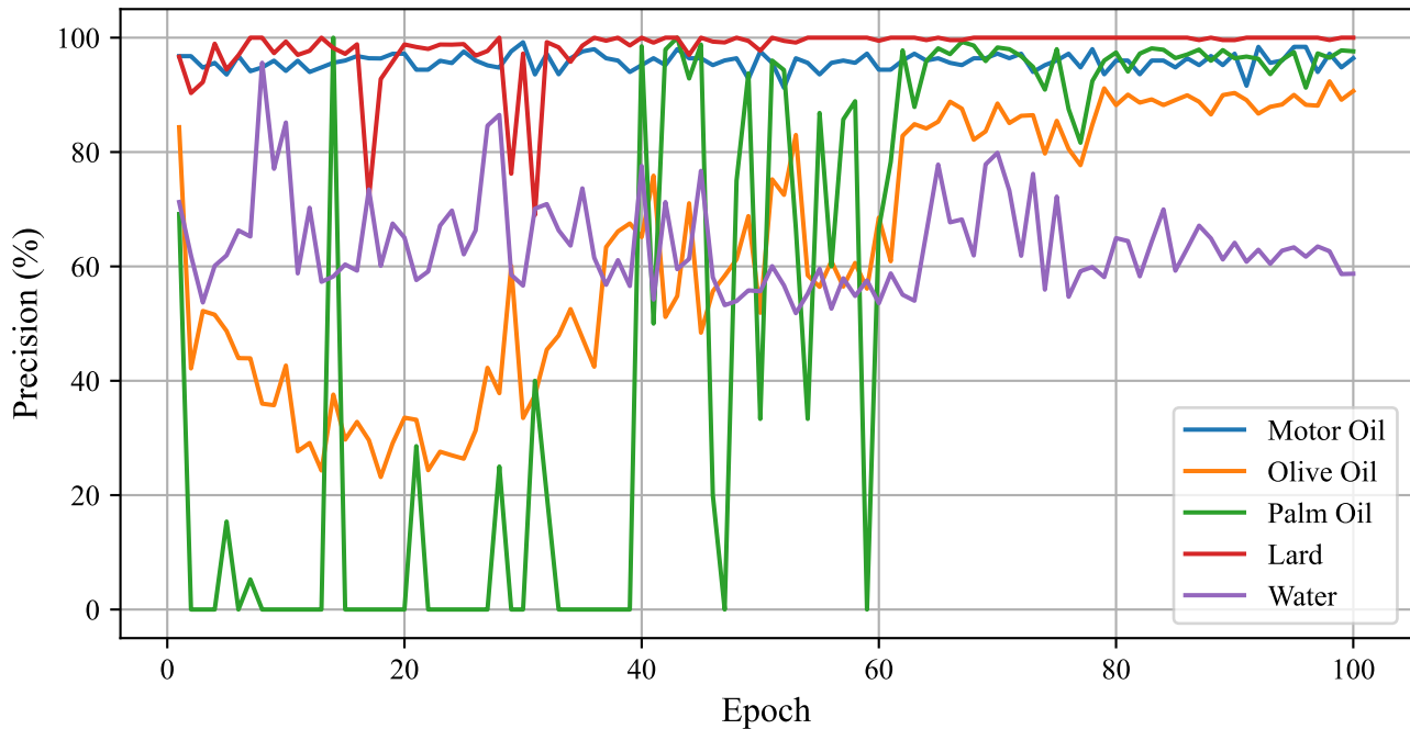
Class Precision
