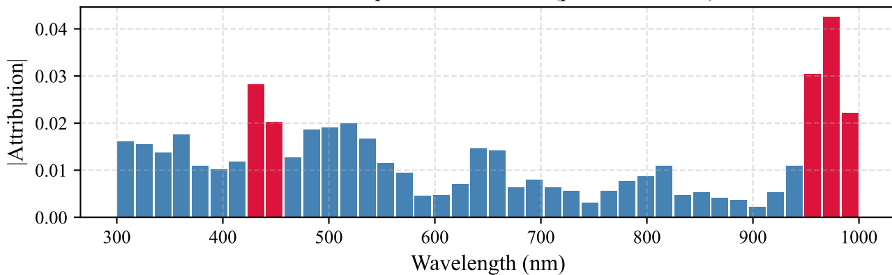
IG Band Importance — Lard (predicted: Lard)
