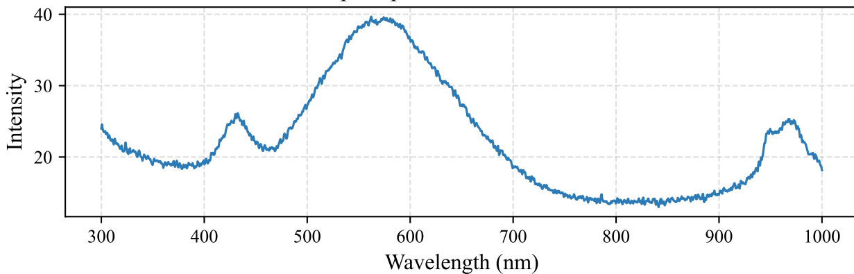
Input Spectrum — Motor Oil
