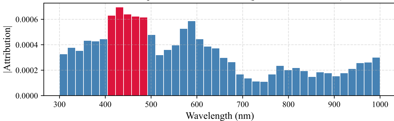
IG Band Importance — Motor Oil (predicted: Motor Oil)
