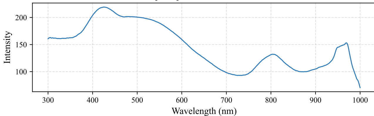
Input Spectrum — Palm Oil
