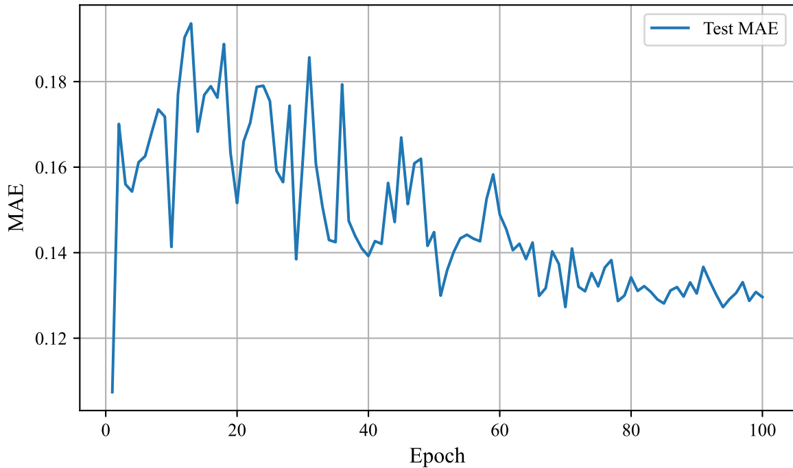
Test MAE Curve
