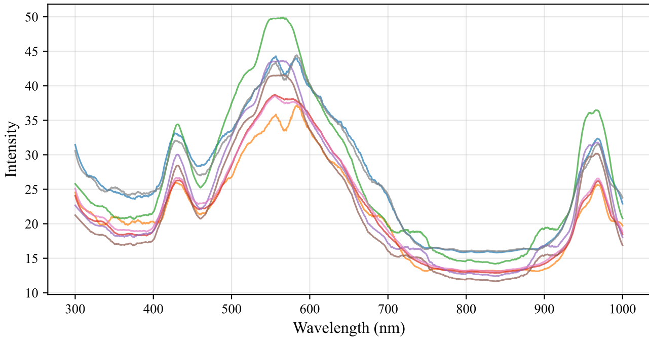
Motor Oil — CGAN Generated Spectrum
