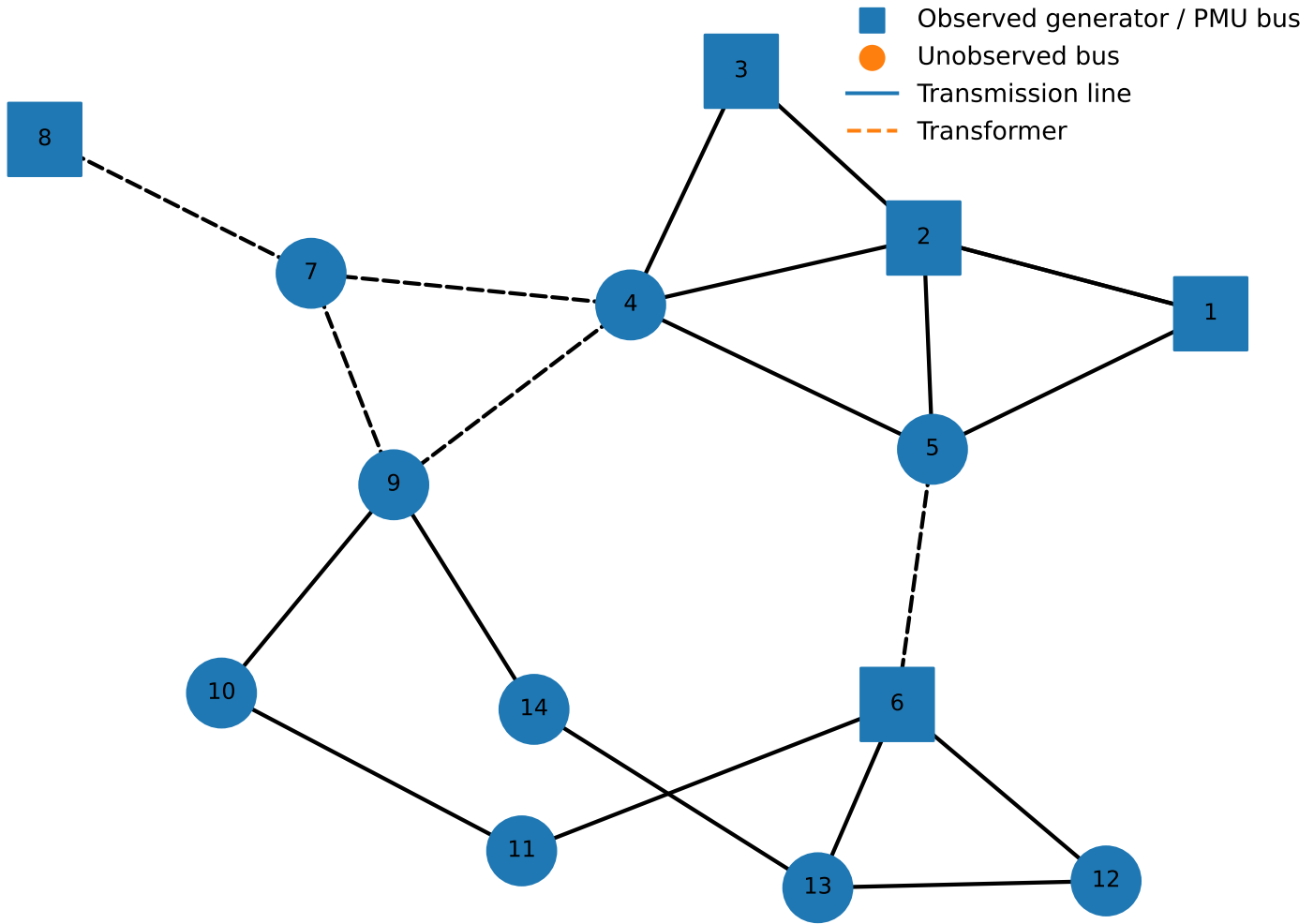
IEEE-14 network and observed generator buses
