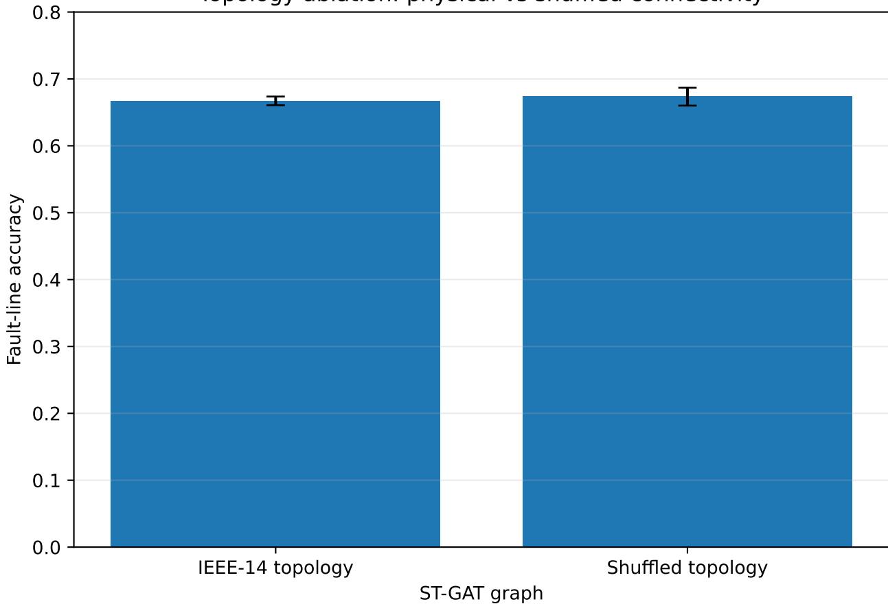
Topology ablation: physical vs shuffled connectivity
