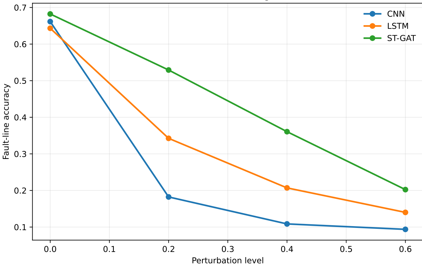
Fault-line localization under missing PMU observations
