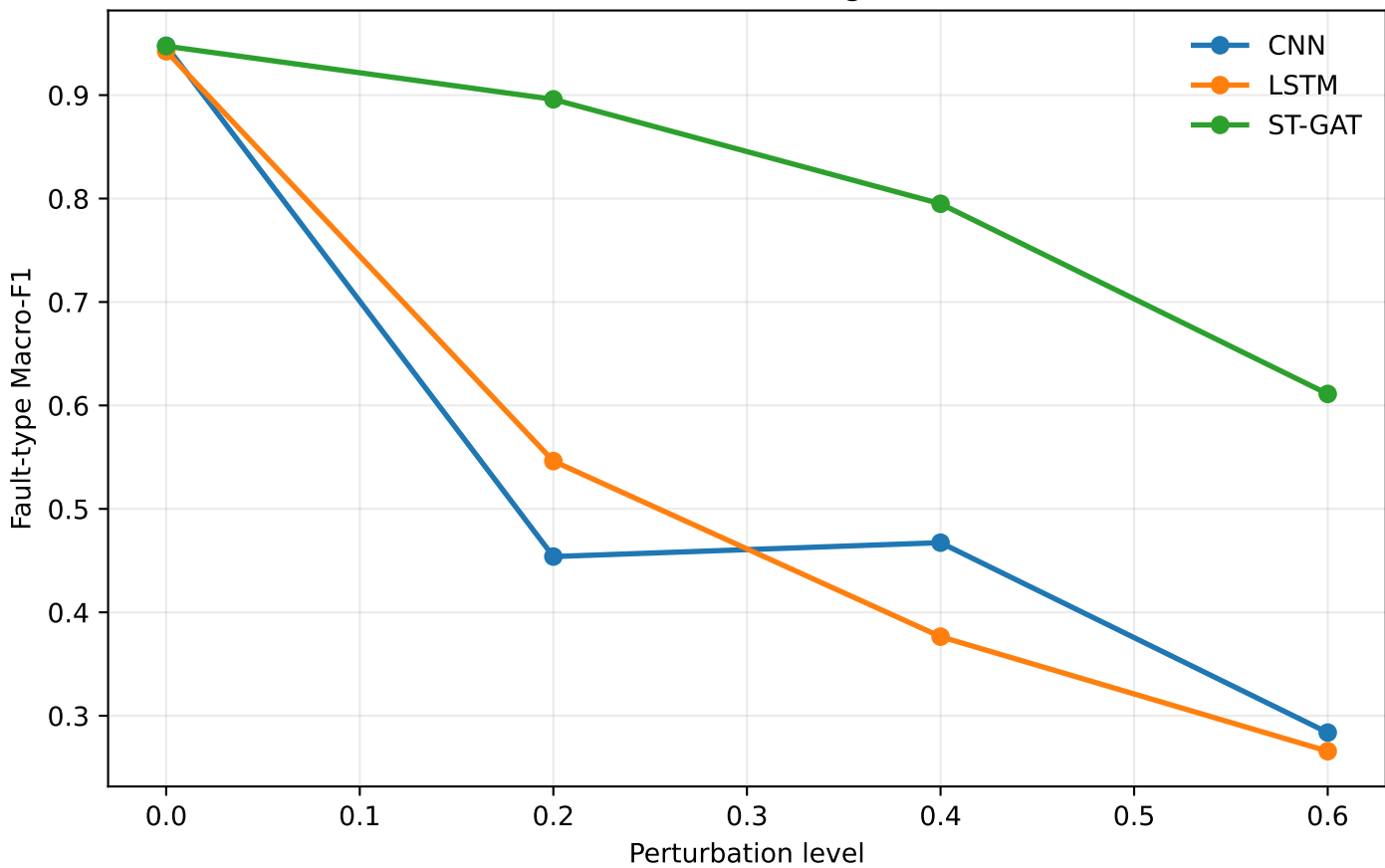
Fault classification under missing PMU observations
