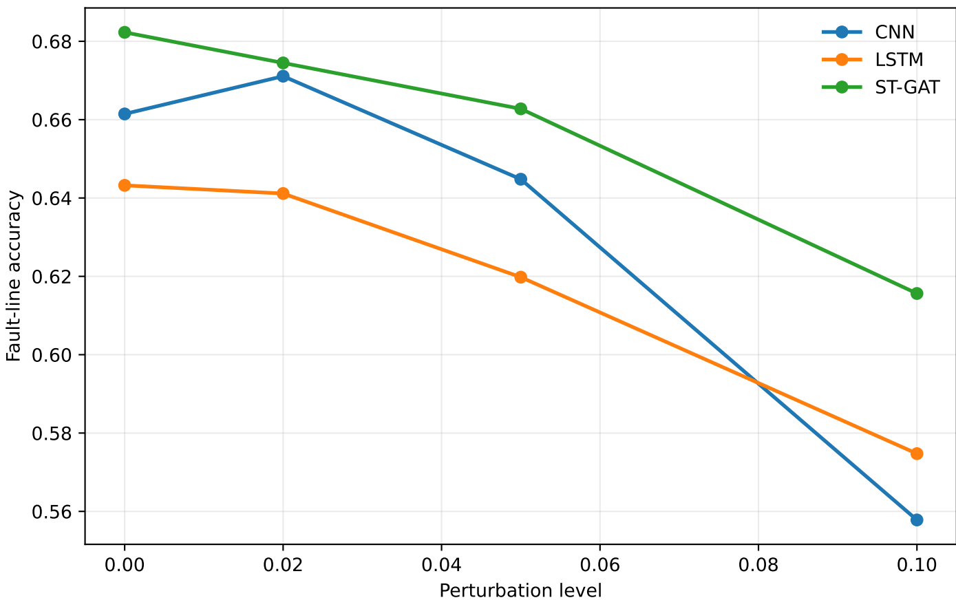
Fault-line localization under Gaussian measurement noise
