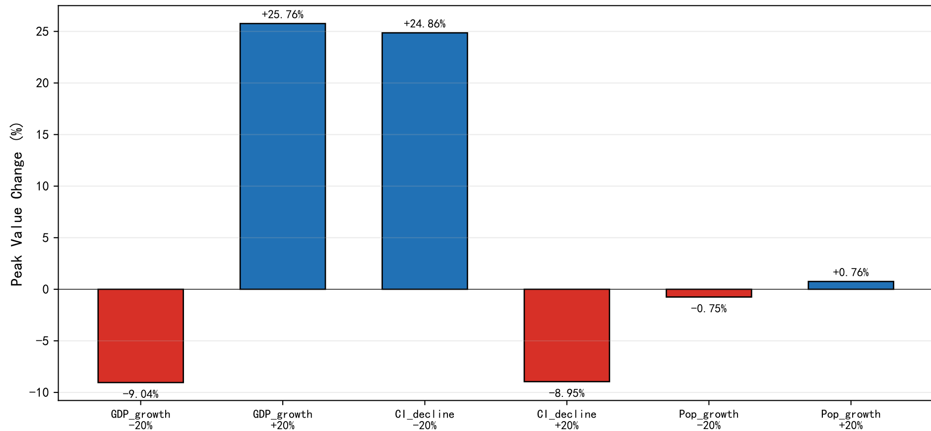
Sensitivity: Parameter Perturbation \pm 20\% on Peak CO2
