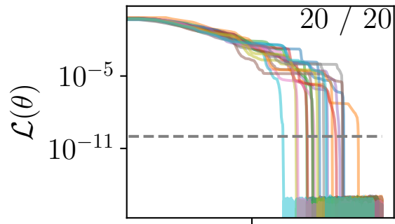
n = 3 No shuffle
