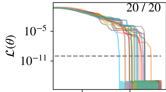
n = 3 no shuffle
