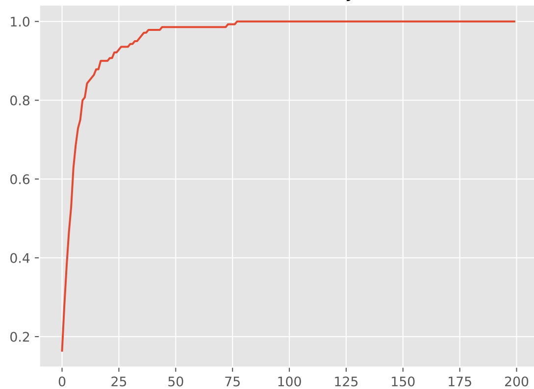
Train accuracy
