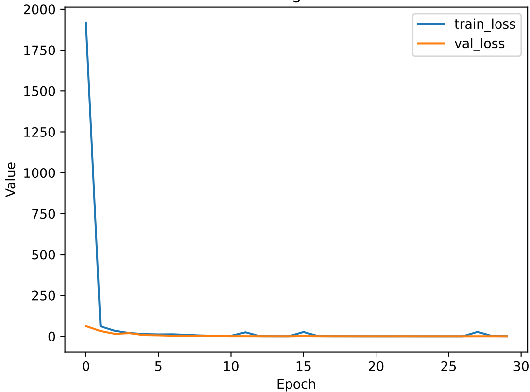
Training Curve
