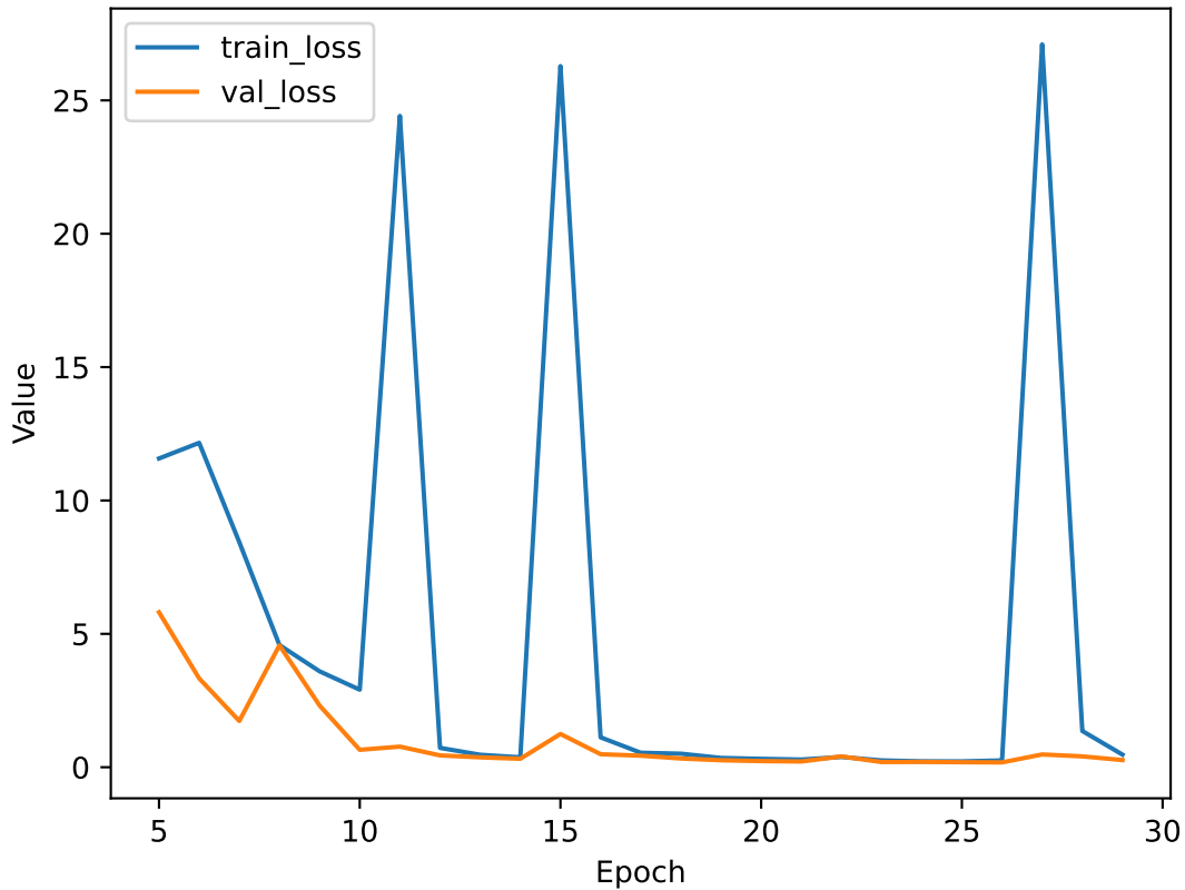
Training Curve
