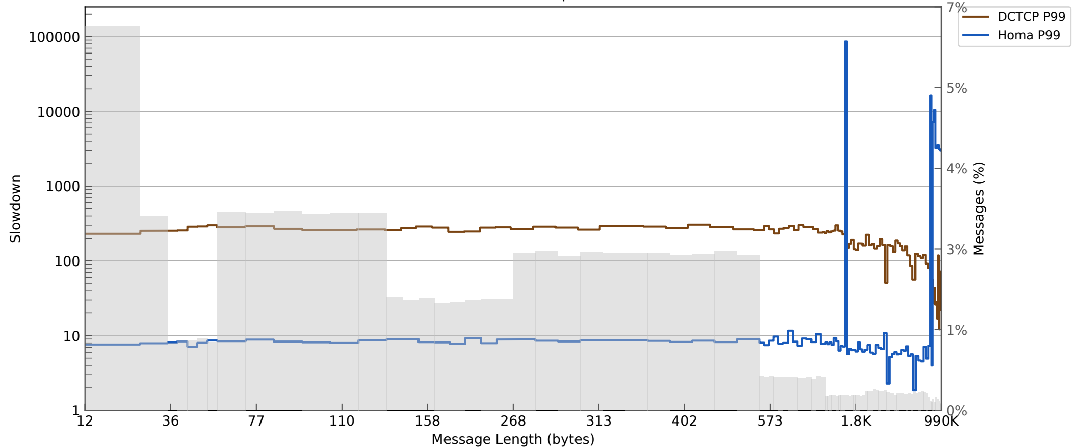
W3 5 nodes, 14.0 Gbps P99
