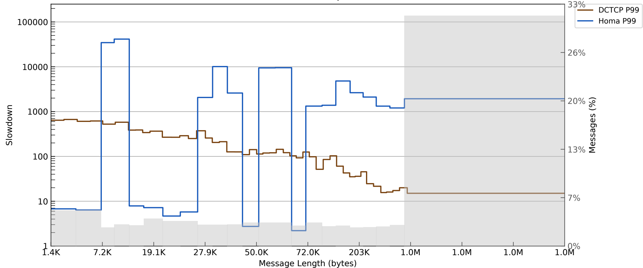
W5 5 nodes, 20.0 Gbps P99
