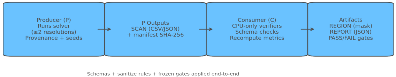
Figure 1. Verification pipeline: Producer (P) generates SCAN artifacts; Consumer (C) re-computes metrics, validates schemas/hashes, and emits REGION + REPORT under frozen gates. All PASS/FAIL results must be reproducible from SCAN alone (single source of truth).
