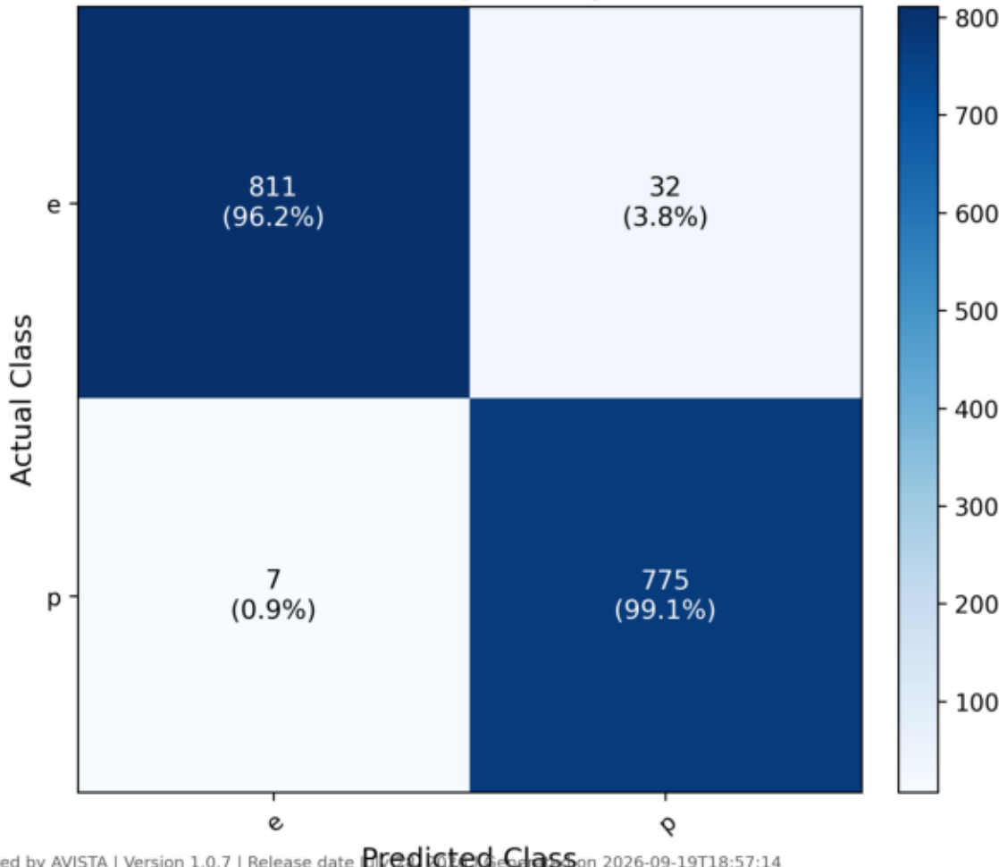
Confusion Matrix - Logistic Regression - Test
