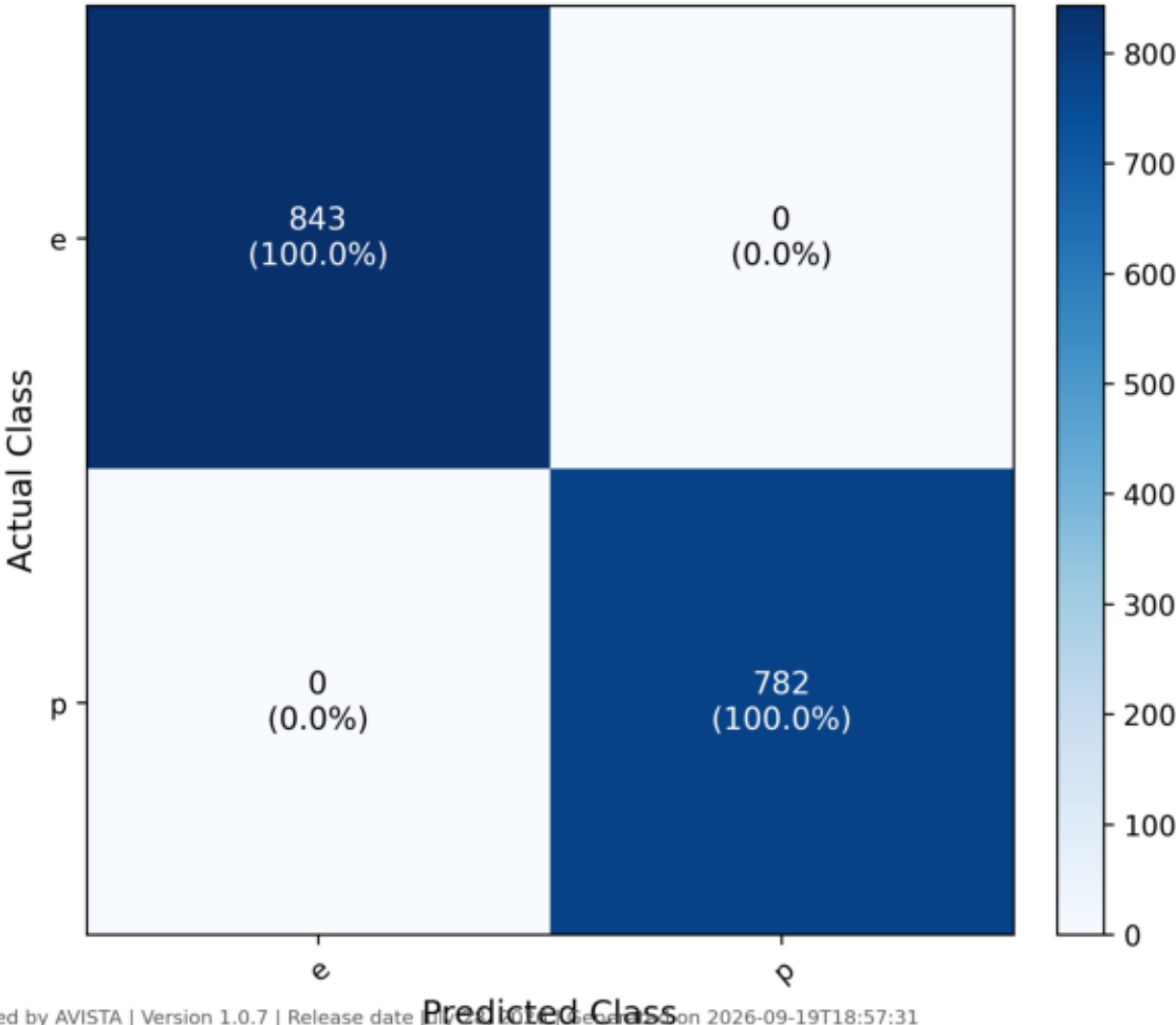
Confusion Matrix - XGBoost - Test
