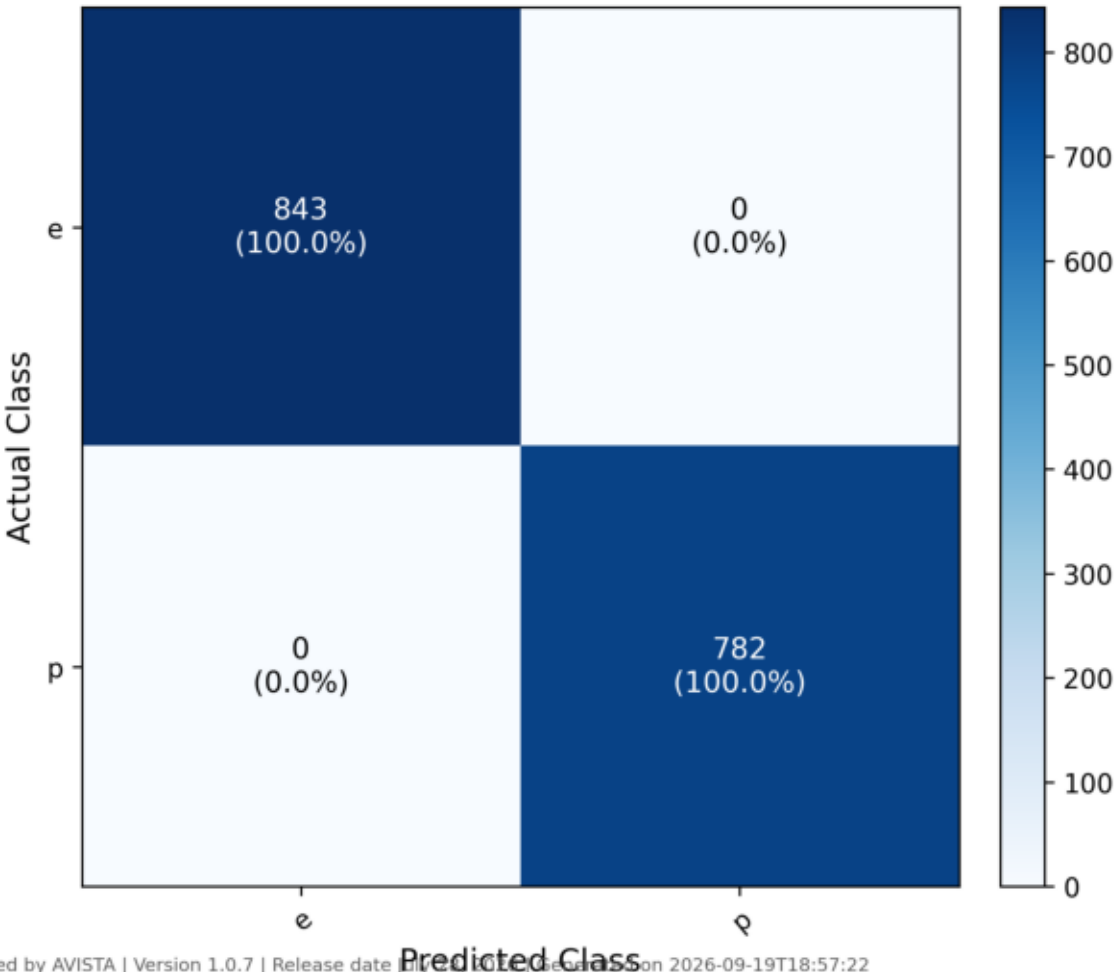
Confusion Matrix - Random Forest - Test
