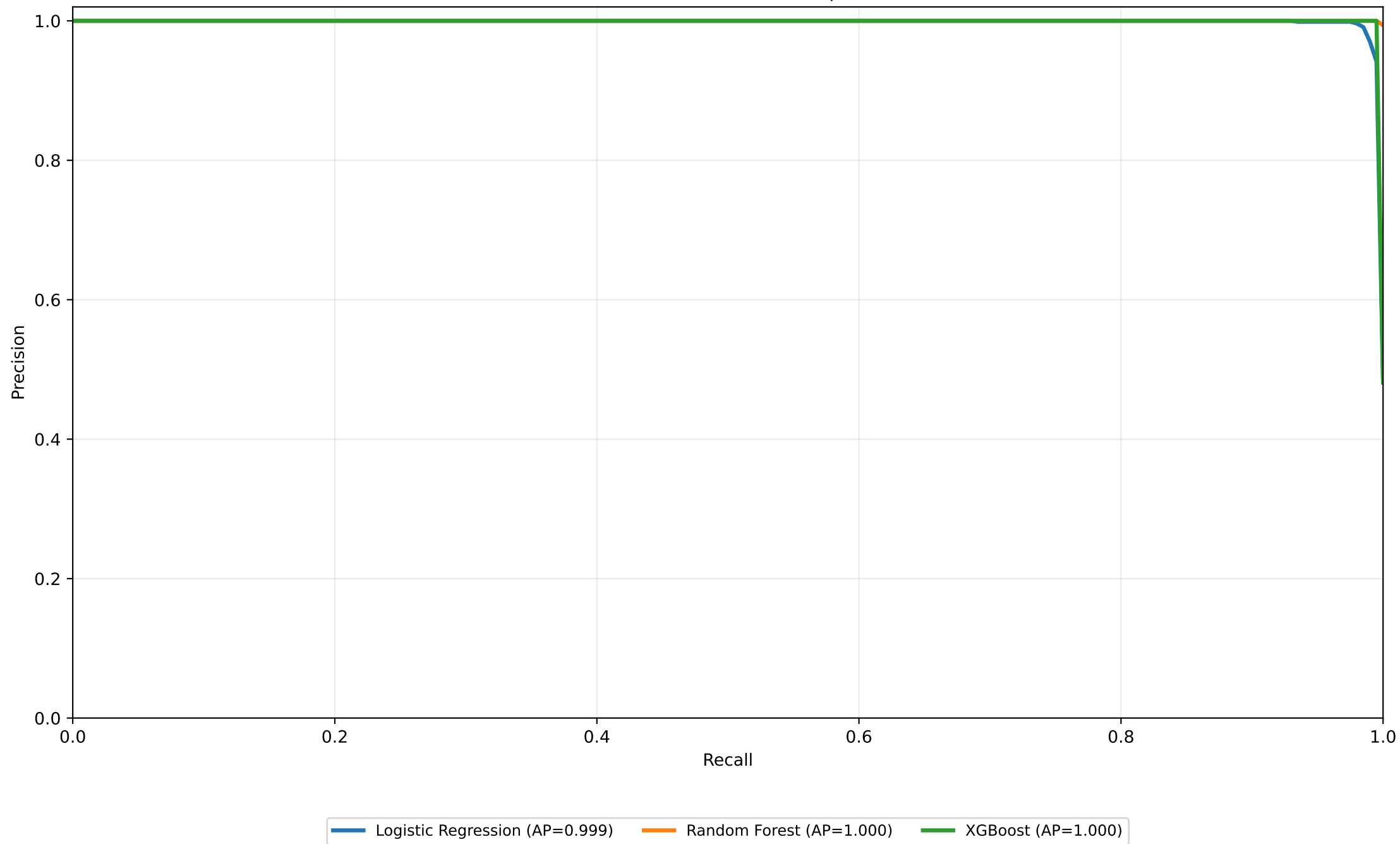
Precision-Recall Curve Comparison
