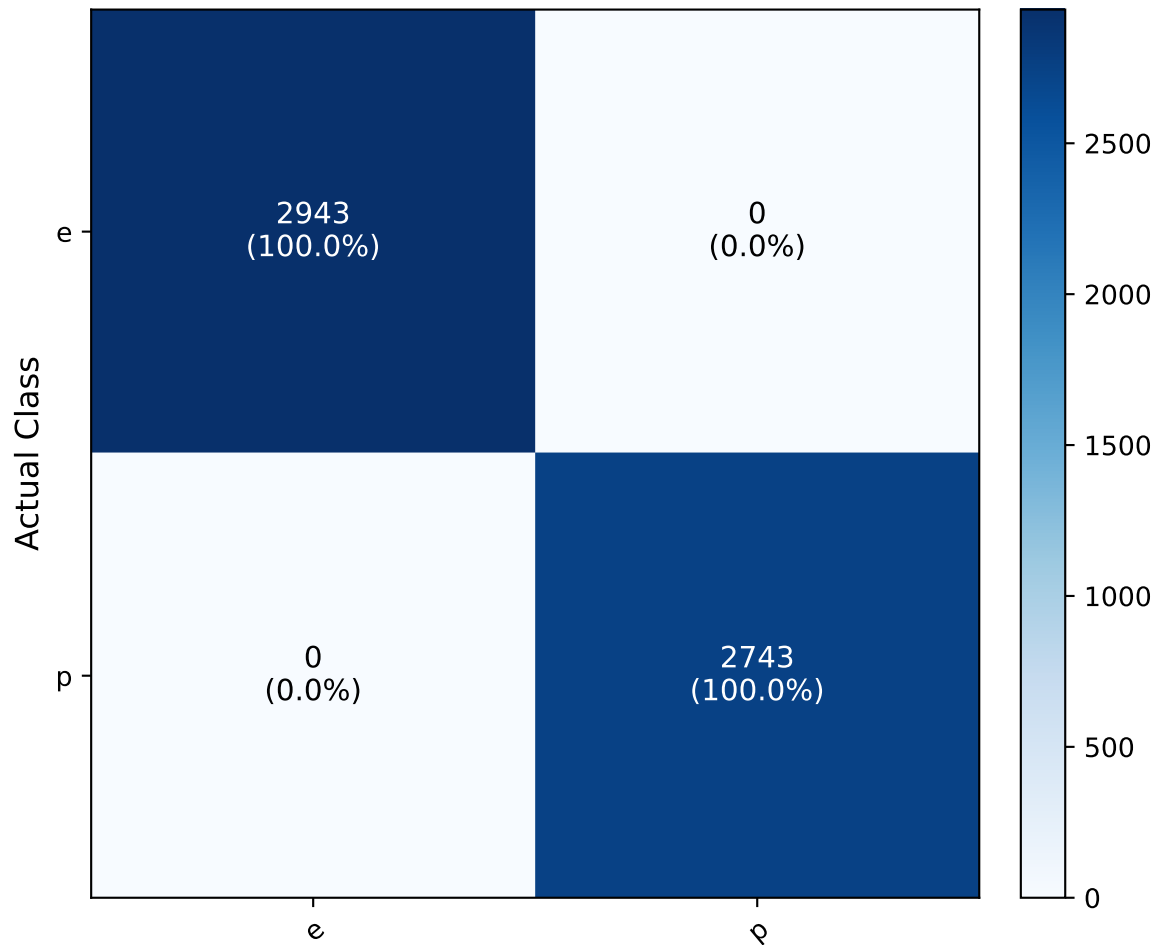
Confusion Matrix - XGBoost - Train
